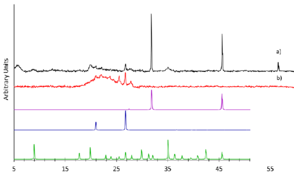
XRD diffractograms: a) Pure Diatomite, b) Acid treated Diatomite, c) Reference pattern of NaCl Halite (PDF-00-001-0993), d) Reference Pattern of SiO 2 Quartz (PDF-01-083-2466) and e) Reference pattern of KAl 2 (AlSi 3 O 10 )(OH) 2 Muscovite (PDF-00-001-1098), Lara et al. pp. 198-209
